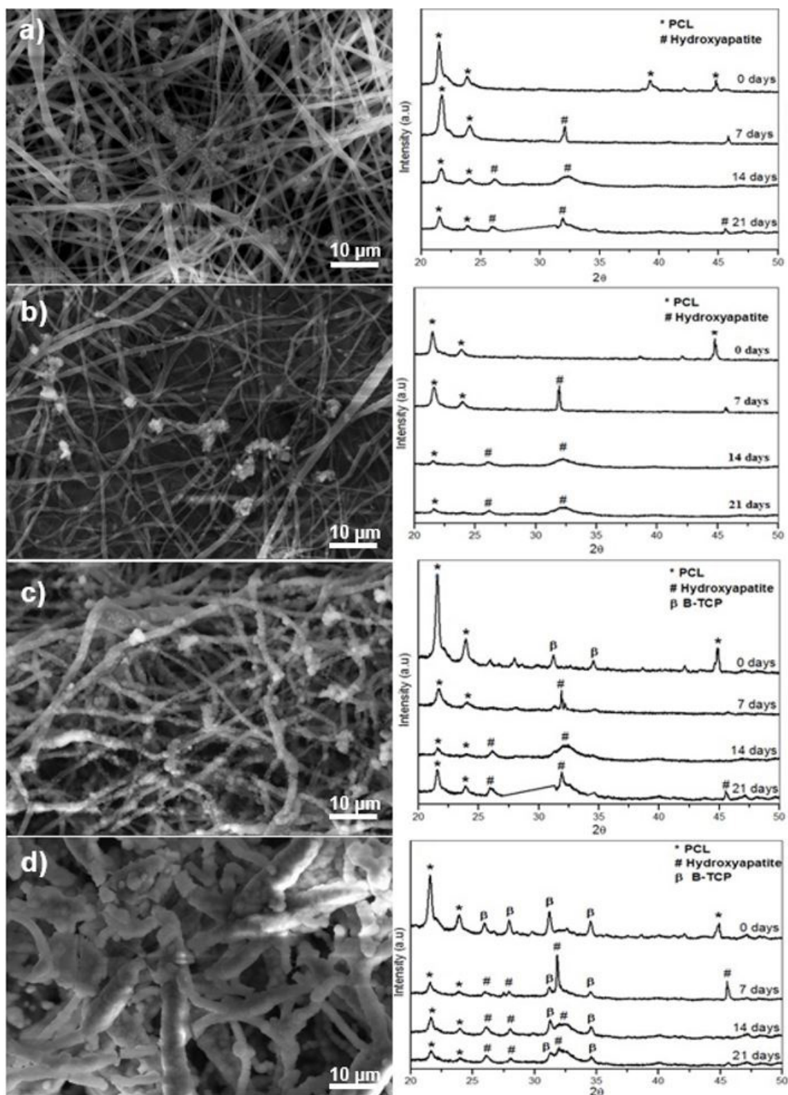
Figure 4. Micrographs of the fibers: (a) PCL; (b) PCL/ \beta -TCP 1 wt-%; (c) PCL/ \beta -TCP 5 wt-%; and (d) PCL/ \beta -TCP 8 wt-% after biomimneralization for 21 days. Right: XRD patterns.
